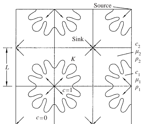
FIGURE 1. The quarter five-spot arrangement of injection and production wells.
