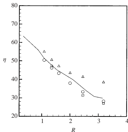
FIGURE 7. Displacement efficiency as a function of the viscosity ratio. —, experimental data by Habermann (1960) and \square , Zhang, Sorbie & Tsibuklis (1997) are compared with \Delta , numerical two-dimensional data for Pe = 800 (obtained with the present three-dimensional code using two-dimensional initial perturbations), and with \circ , the present three-dimensional data for Pe = 800 . The three-dimensional results exhibit significantly better agreement with the experimental data.
