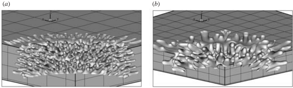
FIGURE 13. Concentration iso-surface for Pe = 1, 200 , G = 0.5 , R = 2.5 and A = 1/8 . A higher instability mode at this value of the Péclet number leads to the generation of small scales. Vigorous fingering starts very early in the simulation. Secondary instability in the form of tip splitting occurs throughout the displacement process. (a) t = 0.04 , (b) t = 0.12 .
